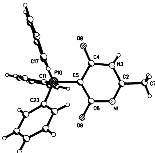
Fig. 1. Molecular Structure of Ylide-Betaine 7a
